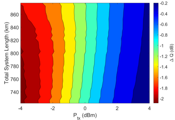
Figure 7. Q calculated from averaged BER compared to a reference system of the same total length
