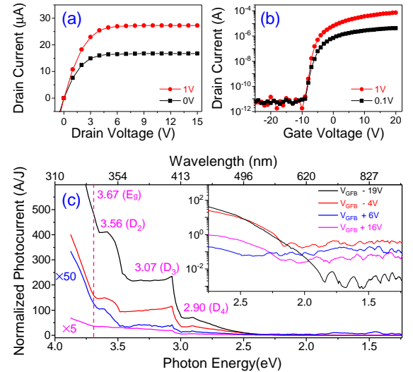
FIG. 1. Transistor data for the a-ZTO TFT. (a) output characteristic and (b) transfer characteristic. The active semiconductor channel W/L ratio was fixed to 38. (c) Normalized photoconducance spectra of the a-ZTO TFT under ps-laser pulsed excitation measured at different V_{GFB} = V_{GS} - V_{FB} . Inset in (c) a semilogarithmic plot of the same photoconductivity spectrum on a magnified scale.
