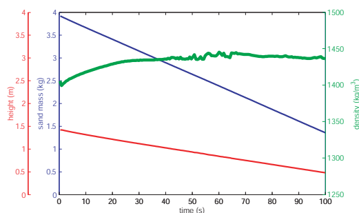
Figure 8. Mean surface height, particle mass, and density during the flow of sand particles in a perspex tube through a gap width of 10mm.
