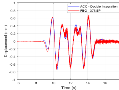
Fig. 7. Span opening at the top of the Arch 37 piers under the Class 185 train load, obtained from FBG and ACC data
