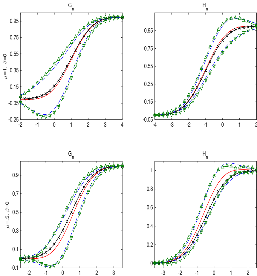
Figure 2. Simulation results for G_n (left) and H_n (right) for design \mu = 1, \beta = 0 (top) and design \mu = 0.5, \beta = 0 (bottom). Each plot contains the mean of the point estimator (solid red line) and the mean of the estimated 95% confidence bands (dashed blue lines), along with the true curve (solid black line, marked \times ) and 95% confidence bands constructed using the Monte Carlo standard deviation (dashed green lines, upper band marked \triangle and lower band marked \nabla ).
