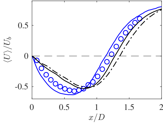
Figure 4: Variation of \langle U \rangle / U_b for the isothermal LES calculations (lines) and measured data ( \circ ) [19] along the centreline. (—) represents the results from PRECISE-MB, and (---) and (—) represent the results from PRECISE-UNS using the constant Smagorinsky model and revised Vreman approach.
