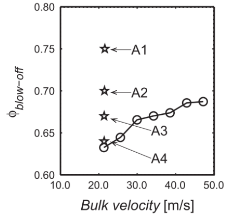
Figure 2: Blow-off curve [18, 19].
