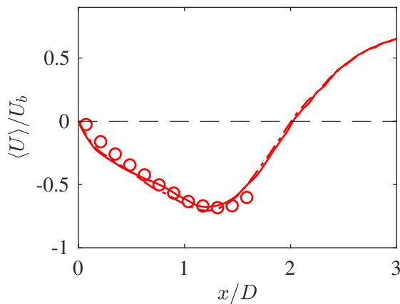
Figure 7: Variation of \langle U \rangle / U_b for the reacting computations performed using PRECISE-MB (lines) and measured data ( \circ ) [19] along the centreline. (—) and (---) represent constant and dynamic \beta_c approaches respectively.
