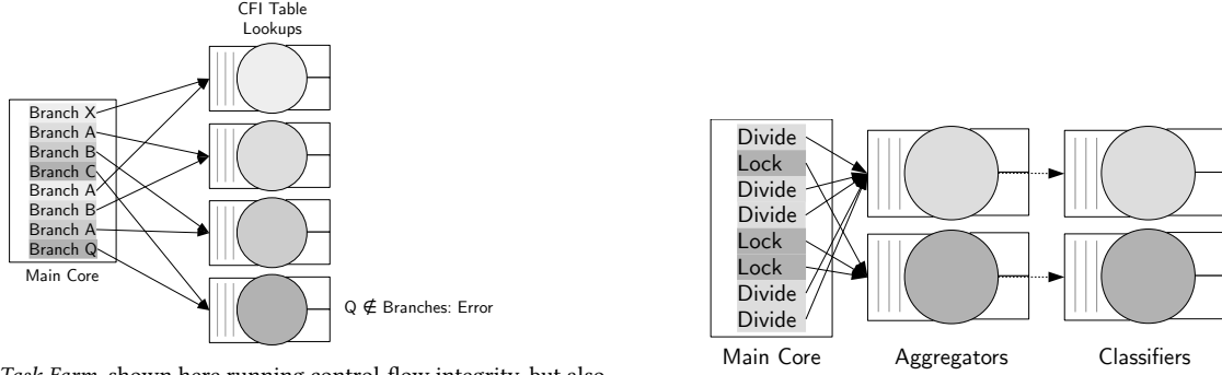
(a) Cyclic Task Farm , shown here running control-flow integrity, but also used for differential fault analysis prevention, reference checker, spatial safety and Rowhammer. Observations are interleaved between the GPEs, and each checked in parallel. (b) Parallel Pipelines , shown here running a covert channel detection mechanism. Each type of event is sent to a single GPE, which then aggregates this information to send to a classifier GPE, in a pipeline formation.
