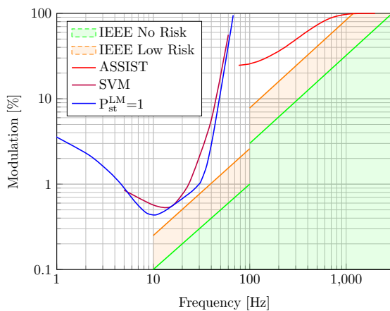
Figure 3: Limits for human perception of flicker, according to different models : ASSIST by Rensselaer Polytechnic Institute, the IEEE and SVM/ P_{st}^{LM} by the IEC. Below the curves, flicker is invisible to the human eye. The shaded areas give an approximate risk assessment for health issues caused by exposure to flicker. The human nervous system is most sensitive to flicker in the range of 10 < f < 50 Hz, as can be seen from the curves. The P_{st}^{LM} = 1 curve has been adopted as a minimum performance limit in EU Regulation 2019/2020. It is equivalent to the levels of flicker present in incandescent light bulbs. Sources: [14, 15, 16].
