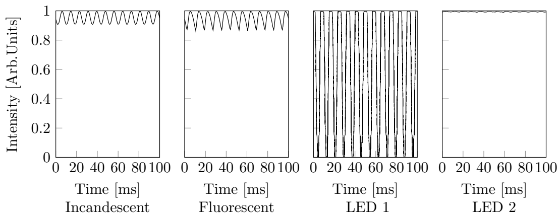
Figure 2: Time-dependent light intensity of incandescent, fluorescent and two different LED light bulbs. The incandescent bulb shows little modulation in its light intensity and thus good flicker performance. Significant increases in modulation can be seen for the fluorescent bulb. LED 1, equipped with a cheap ballast, displays levels of modulation that cause flicker at a level that is classified as ‘dangerous’ according to the safety guidelines from Figure 3. LED 2, equipped with a more complex and more expensive ballast, shows no visible flicker. Source: [12].
