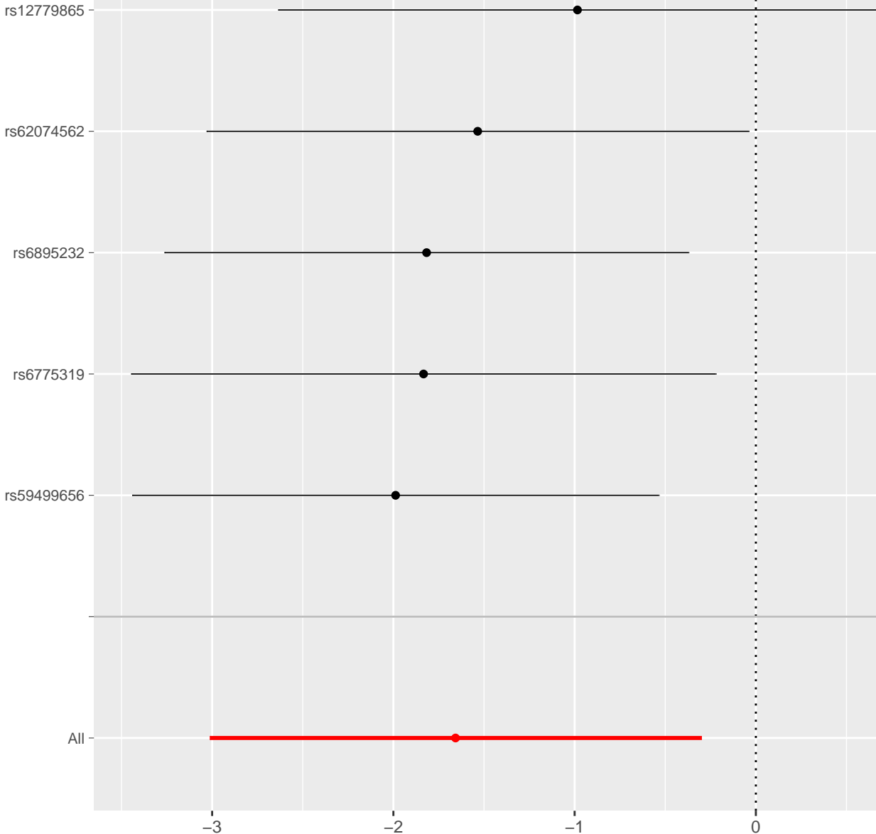
MR leave-one-out sensitivity analysis for 'Physical activity' on 'Severe respiratory COVID-19'
