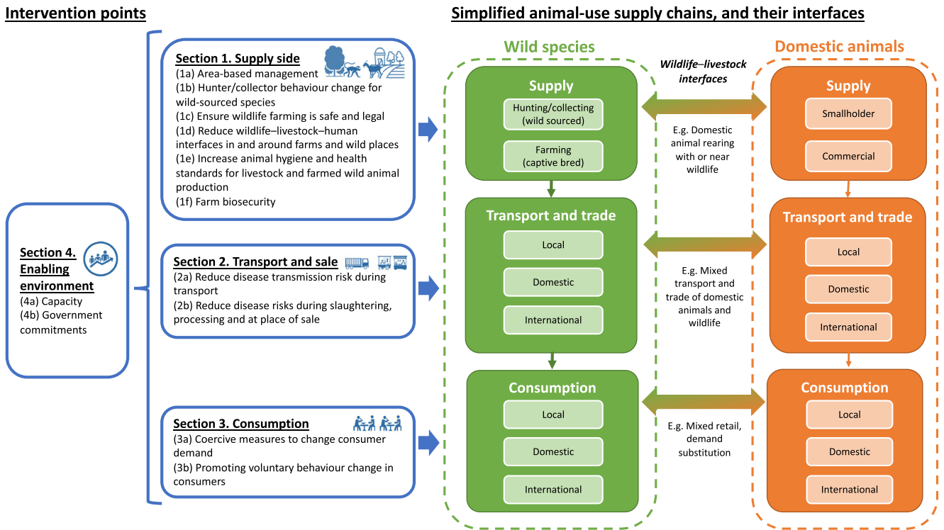
Fig. 1. A conceptual diagram of animal-use supply chains and their interfaces, identifying different intervention points and intervention options at different stages in the supply chain.
