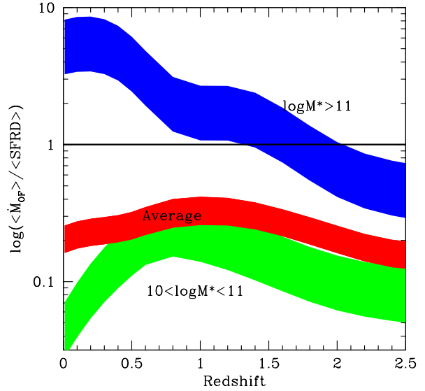
Fig. 12. The average mass-loading factor \langle \eta \rangle = \langle \dot{M}_{OF} D \rangle / \langle SFRD \rangle as a function of the redshift. Red=average; blue= M^* > 10^{11} M_\odot ; green= 10^{10} < M^* < 10^{11} M_\odot .
