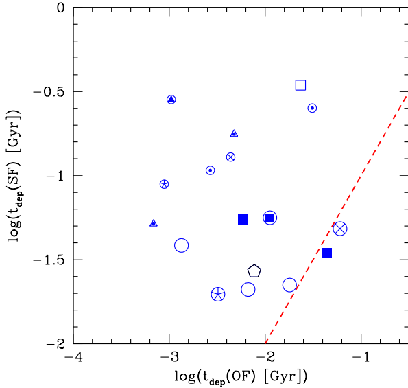
Fig. 8. The SFR depletion timescale, t_{\text{dep}}(SF) = M_{\text{gas}}/SFR , as a function of the wind depletion timescale, t_{\text{dep}}(OF) = M_{\text{gas}}/\dot{M}_{OF} . The red dashed line is the depletion timescale due to star formation at the measured rate.
