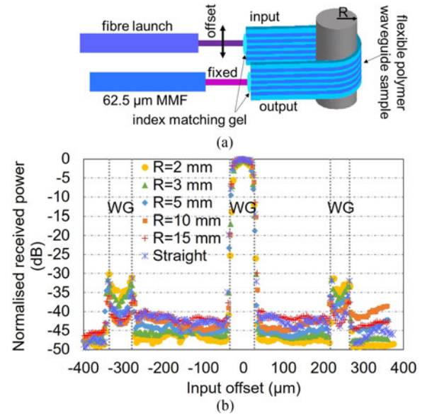
Fig. 10. (a) Schematic of crosstalk measurement of bent waveguide sample and (b) normalised received power at the waveguide output as a function of the input position for different bending radii for the 4 \mu\text{m} SMF input.
