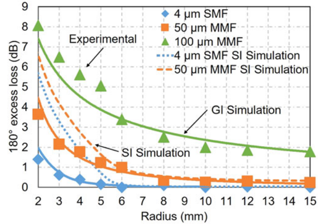
Fig. 5. Excess bending loss for different bending radii, experimental (symbols) and simulation (lines) results.
