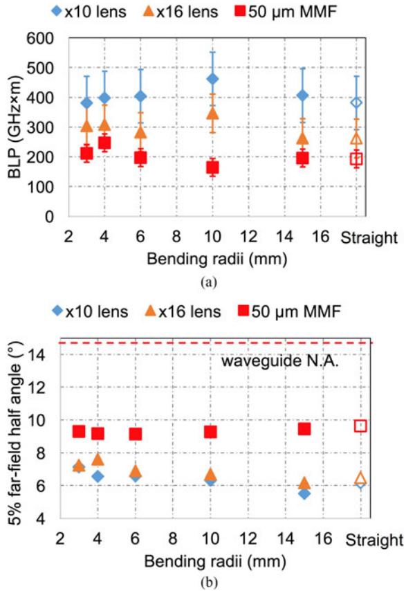
Fig. 17. (a) Bandwidth length product of the flexible polymer waveguide sample and (b) the 5% far-field half angle of the waveguide output laser beam.
