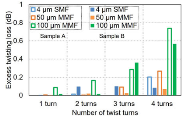
Fig. 14. Average twisting excess loss for samples A and B as a function of the number of full 360° twists for the different launch conditions.
