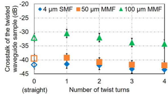
Fig. 15. Crosstalk of a twisted flexible waveguide sample for different numbers of full twisting turns and the different launch conditions (fibre diameters).
