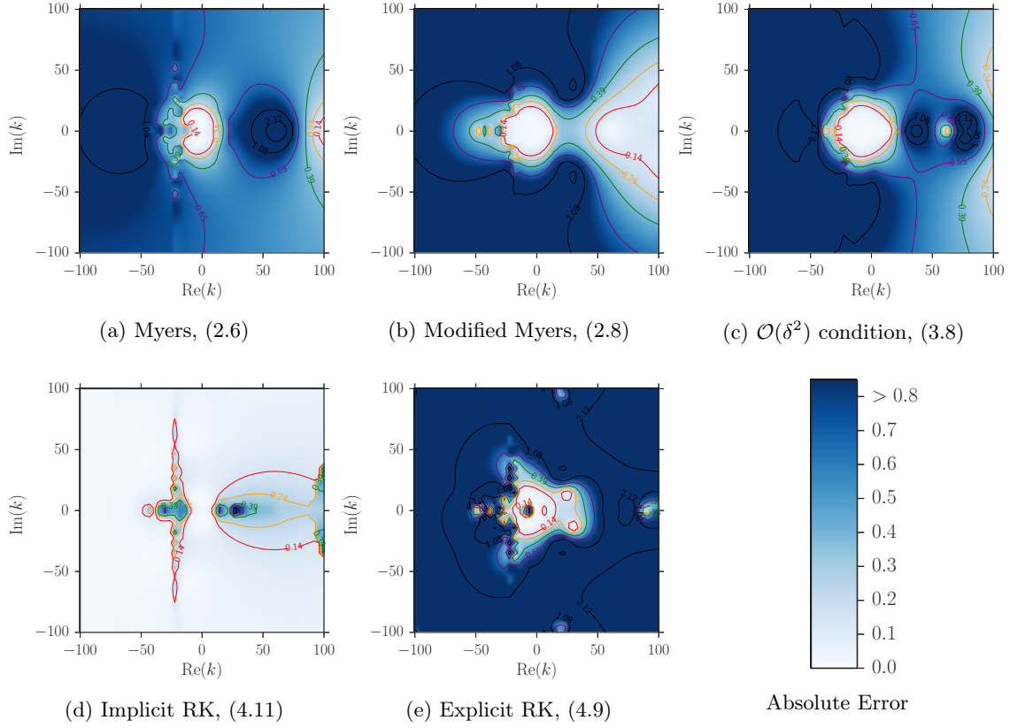
Figure 3. As in fig. 2, but for a boundary layer thickness \delta = 3 \times 10^{-2} . Note also the different error scale compared with fig. 2.
