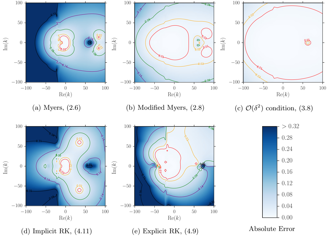
Figure 2. Absolute errors in the complex k -plane of the predicted Z_{\text{eff}} for each boundary condition. The colour scheme is normalised such that the darkest blue is an error greater than or equal to 1.5 times the mean Myers error. The red contour surrounds errors lower than the lowest quartile of the combined results for the Myers, Modified Myers, second order asymptotic and the single-step implicit Runge-Kutta conditions. Error was calculated as \min\{|Z_1 - Z_2|, |1/Z_1 - 1/Z_2|\} . Parameters are \omega = 31 , m = 24 , M = 0.5 , \delta = 2 \times 10^{-3} , for a tanh velocity profile (5.1) and constant base density \rho(r) \equiv 1 . The boundary impedance at each point is found from the numerical solution of the Pridmore-Brown equation, (2.3a).
