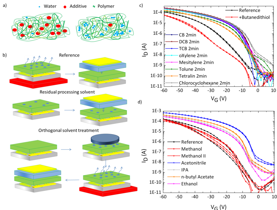
Figure 1 Effect of water removal through azeotrope solvents on the performance of OFETs (a, left panel) Passivation of water induced traps in the polymer's microstructure (green) through the use of additives (red); (a, right panel) Removal of additives allows water molecules (blue) to interact with polarons on the polymer backbone and disturb charge transport (b) Method of water removal in IDT-BT OFETs ( L = 20\mu m , W = 1mm ); (i) Reference top gate device with the polymer film (green) initially containing residual solvent (blue) after spin-coating. Annealing at 100 C on a hotplate (red) for 1h removes the residual solvent. This is followed by the deposition of the dielectric (blue) and gate (yellow); (ii) Device prepared with residual solvent being deliberately left in the polymer film. Only a short anneal for 2 minutes is used which removes most of the solvent, but leaves residual solvent filling voids in the film; (iii) Devices prepared under conditions in which the annealed polymer film is soaked in an orthogonal solvent and subsequently annealed at 100°C for 1h; c) Saturation ( V_{DS} = -50V ) transfer characteristics of an annealed reference device (black) and devices with residual azeotrope and zeotrope solvents processed according to (ii); (d) Saturation transfer characteristics of devices treated with orthogonal solvents according to (iii). Devices treated with methanol (zeotrope) were reproduced several times with 2 devices from different batches shown.
