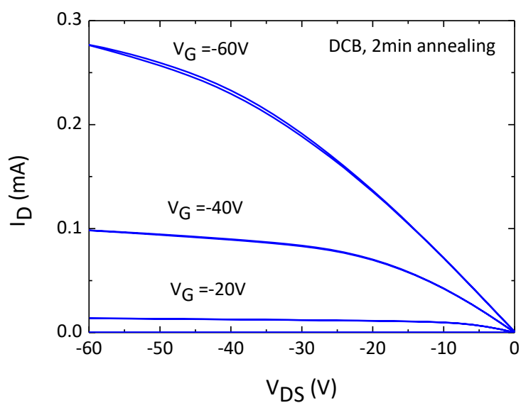
Fig. S2 Output characteristics of an IDTBT OTFT ( L=20\mu m , W=1mm ) processed from DCB and annealed for 2 minutes only leaving residual solvent in the film that can hydrogen bond to water molecules in the film and form an azeotrope.
