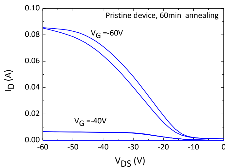
Fig. S1 Output characteristics of a pristine IDTBT OTFT ( L=20\mu m , W=1mm ) processed from DCB and annealed for 60 minutes.
