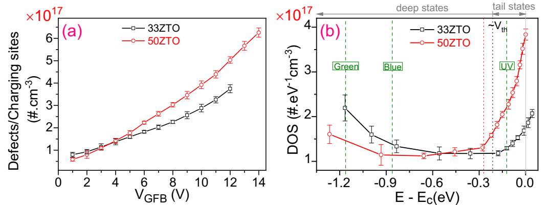
Figure 7. (a) The extracted sub-bandgap defects/charging sites density as a function of V_{GFB} ( =V_G - V_{FB} ) for 33ZTO and 50ZTO TFTs. (b) The extracted density of sub-bandgap states (DOS) versus E - E_c (eV).
