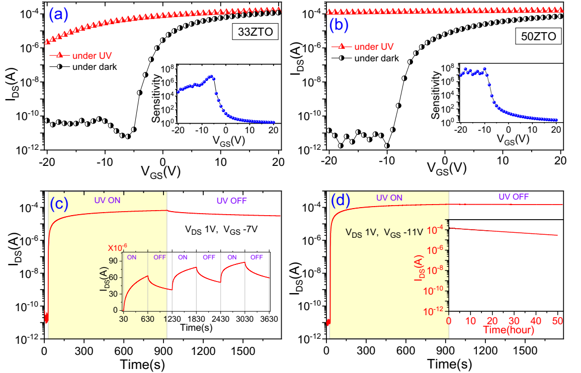
Figure 3. The transfer characteristics of (a) 33ZTO and (b) 50ZTO TFTs at V_{DS} = 1 \text{ V} measured in dark and under UV light (at 365 nm) exposure. The sample was exposed to UV light for 5 min at an intensity of 40 \text{ mW/cm}^2 before starting the photocurrent-voltage measurement. Insets show the sensitivity (photo-to-dark current ratio) as a function of V_{GS} . In (c) and (d), the transient response of the drain-to-source current for ZTO photo-TFTs under a single UV light pulse of 15 min for the sample 33ZTO and 50ZTO, respectively. The inset in (c) shows photoresponse of 33ZTO under a periodic UV pulse (10 min). The inset in (d) shows extended measurement (up to 50 hrs) of drain-to-source photocurrent after switching off the UV light.
