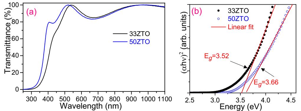
Figure 2. (a) UV-Vis transmission spectra and (b) calculation of the bandgap energy of the ZTO thinfilms on Corning glass substrate with an elemental composition identical to semiconductor channels of 33ZTO and 50ZTO TFTs.
