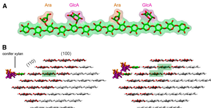
Figure 11. Cellulose-xylan complexes used for molecular dynamics simulations. A, Conifer xylan model. B, Cellulose microfibril with one and two conifer xylans docked onto the (110) face. Only the dark-gray part of the cellulose was considered in the simulations to save computational cost. Highlighted in green are the glucan chains that were replicated and translated to the cellulose surface to build the xylan chains.
