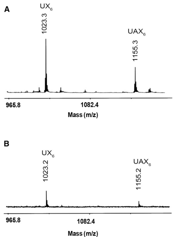
Figure 4. Mass spectrometry of glucuronoxylanase GH30 digestion products of conifer xylan. A, MALDI-ToF-MS of glucuronoxylanase GH30 digestion of NaOH-extracted, deacetylated Douglas fir xylan shows two species UX 6 and UAX 6 . B, MALDI-ToF-MS of glucuronoxylanase GH30 digestion of DMSO-extracted conifer xylan shows no acetylation of UX 6 or UAX 6 .
