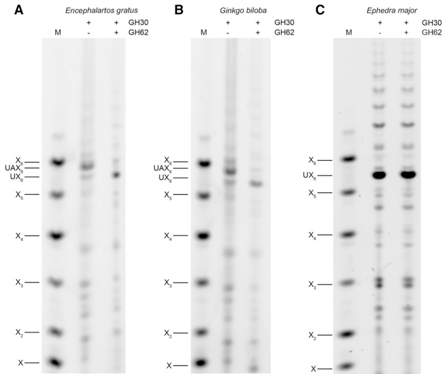
Figure 7. Xylan is decorated with \alpha -arabinofuranose in cycad and Ginkgo but not Gnetophyta. Glucuronoxylanase GH30 digestion products of cycad ( E. gratus ; A), Ginkgo ( G. biloba ; B), and Gnetophyta ( E. major ; C) xylan were digested with \alpha -arabinofuranosidase GH62 and analyzed by PACE. UAX 6 present in cycad and Ginkgo GH30 digestion products is sensitive to the arabinosidase. Marker (M), xylosyl oligosaccharides X 1 -X 6 .
