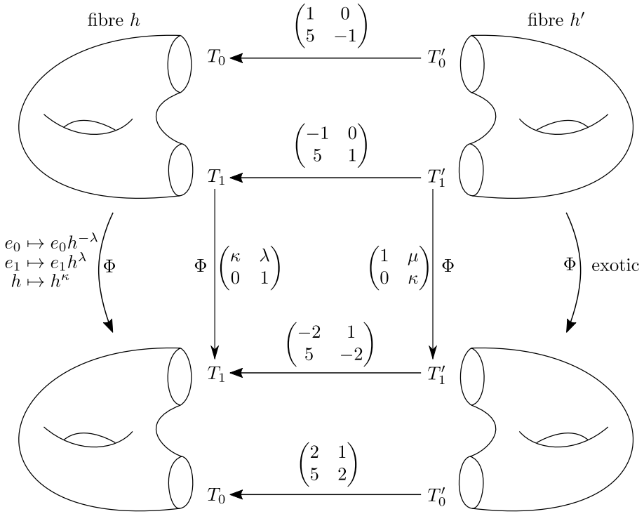
Figure 2. The graph manifolds considered in Example 2.2. Here each Seifert fibered piece is product of a surface with \mathbb{S}^1 . Each boundary subgroup T_i^{(\prime)} is given an ordered basis (h^{(\prime)}, e_i^{(\prime)}) . Please note that for clarity we have swapped the roles of T_0 and T_1 in the lower diagram and omitted the maps induced by \Phi on T_0 and T'_0 .
