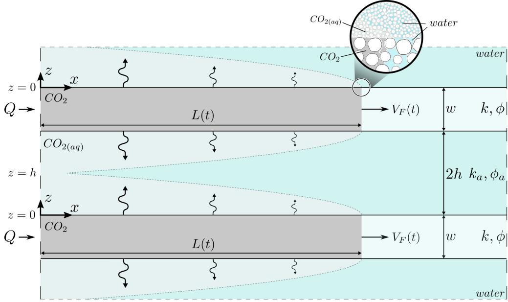
Figure 3. Schematic diagram of periodically repeating high permeability porous layers of width w , separated by low permeability porous layers of width 2h . The reservoir is initially saturated with water. CO 2 is injected into the high permeability layers. z = 0 at the high/low permeability interface and z = h at the midpoint between the high permeability layers.
