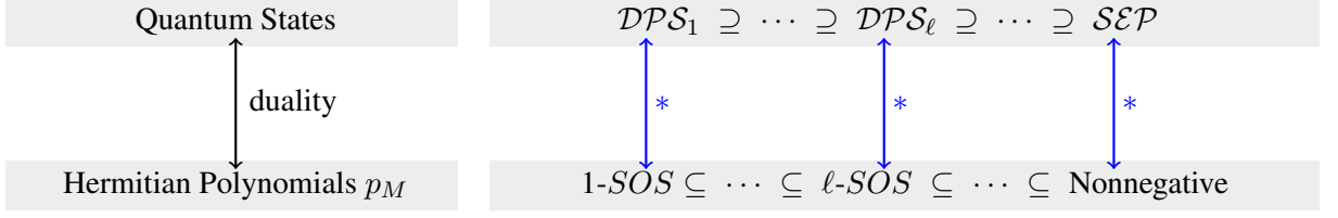
Figure 1: A summary of the duality relations between the DPS hierarchy and sums of squares. The notation \ell\text{-SOS} is a shorthand for \|y\|^{2(\ell-1)} p_M is a real sum-of-squares.
