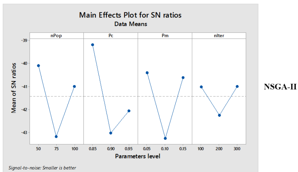
Fig. 9. The mean S/N ratio plot for each algorithm
