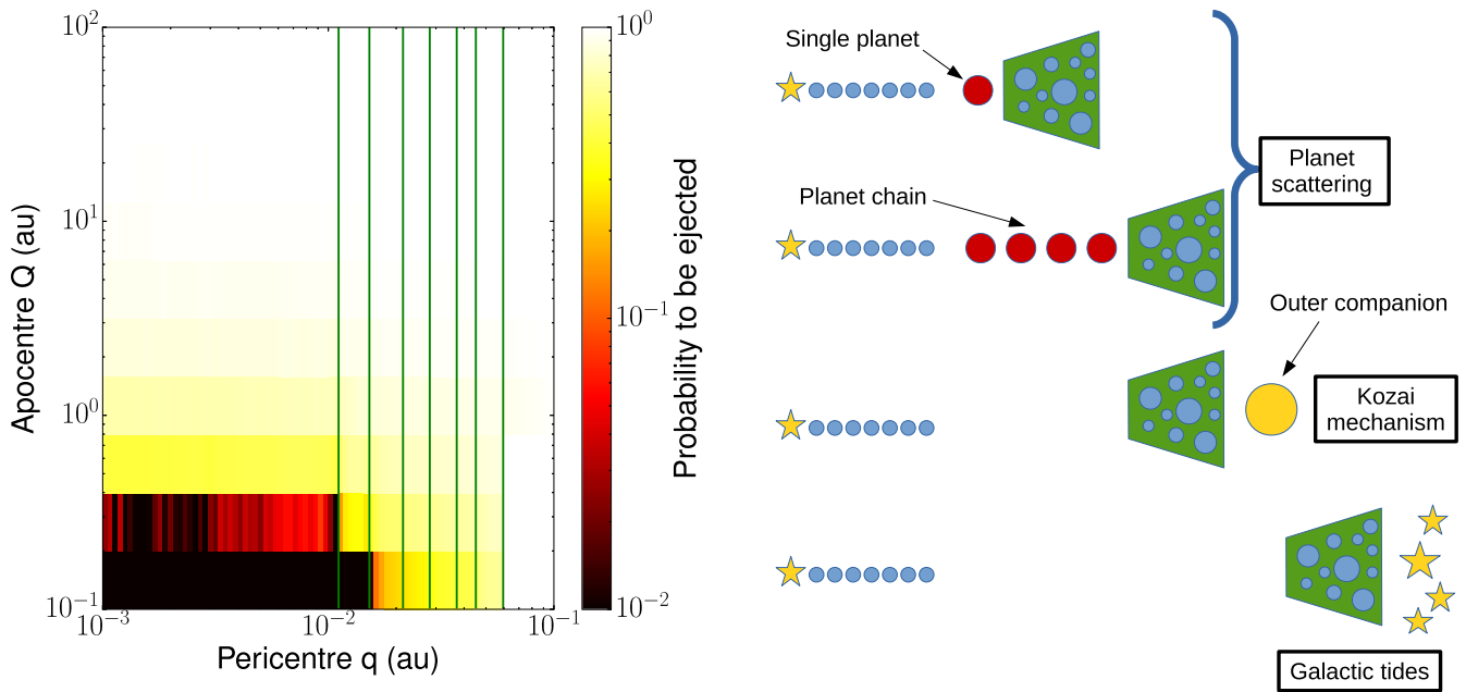
Figure 9. New ejection map: similar to Fig. 3, but for an inclined distribution of comets (see Section 3.5 for more details).
