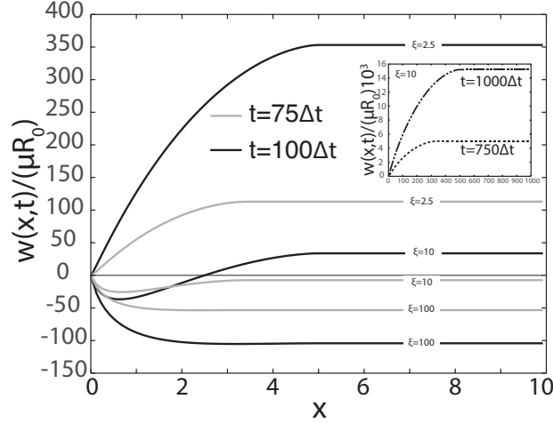
FIGURE 10. Magnitude of the relative w(x,t) displacement \xi under normal ramp loading over different instants in time. We note that for \xi = 10 the solution changes from fully reverse slip to partial reverse slip. Over longer periods of time (inset), the solution becomes entirely forward slip.
