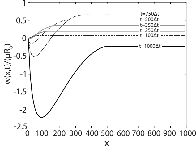
FIGURE 9. Magnitude of the relative w(x,t) displacement \xi = 100 under shock loading over different instants in time. The solution evolves in time from a fully direct slip wave to a reverse stick-slip wave.
