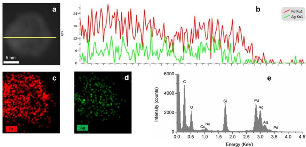
Figure 7. (a-b) EDS line scan of the Ag-Pd hollow NPs, (c-d) EDS elemental mapping of Ag-Pd hollow NPs, (e) EDS spectra of the Ag-Pd hollow NPs after Reactor 3 using \text{Pd}(\text{NO}_3)_2 as precursor.
