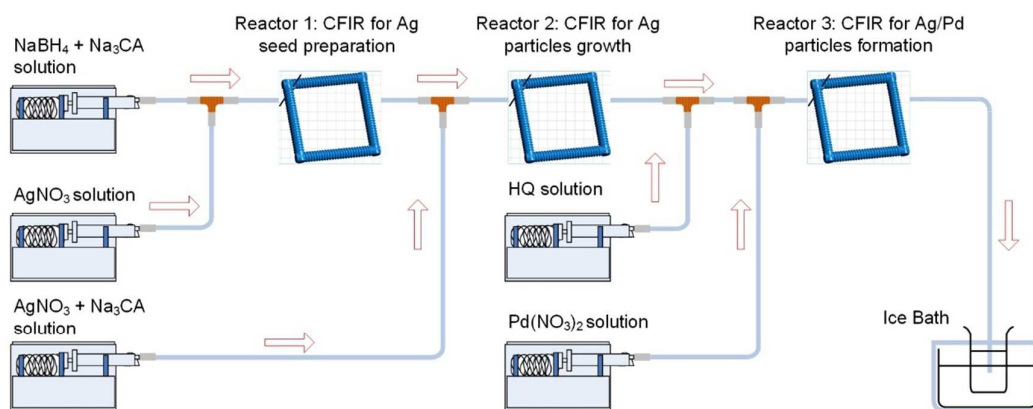
Figure 1. Synthesis of hollow Ag-Pd bimetallic nanoparticles using CFIR reactors connected in series.
