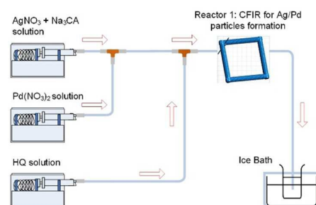
Figure 10. Simultaneous reduction of \text{Ag}(\text{NO}_3) and \text{Pd}(\text{NO}_3)_2 with HQ in a CFI microreactor.
