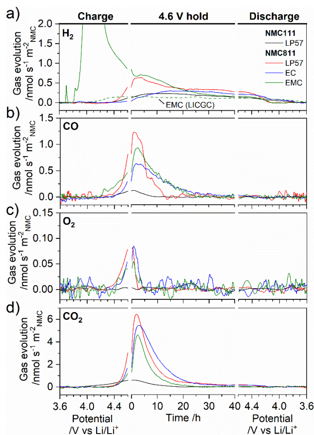
Figure 2. Evolution of (a) \text{H}_2 , (b) \text{CO} , (c) \text{O}_2 , and (d) \text{CO}_2 as determined from the OEMS channels m/z = 2, 28, 32 , and 44 , respectively, and normalized to the NMC surface area. For NMC/Li cells during the first charge-discharge cycle between 2.5-4.6 V at C/20 with a 40 h potentiostatic hold at 4.6 V. For NMC111 with LP57 electrolyte and NMC811 with electrolytes LP57, 1.5 M \text{LiPF}_6 in ethyl methyl carbonate (EMC), and 1.5 M \text{LiPF}_6 in ethylene carbonate (EC). Data are plotted as a function of potential for the charge and discharge, and time for the potentiostatic hold. The evolution of \text{H}_2 for a NMC811/Li cell with a lithium ion conducting glass-ceramic separator (Ohara, LICGC) with 1.5 M \text{LiPF}_6 in EMC as the catholyte and LP57 as the anolyte is also shown in (a) – dashed green line.
