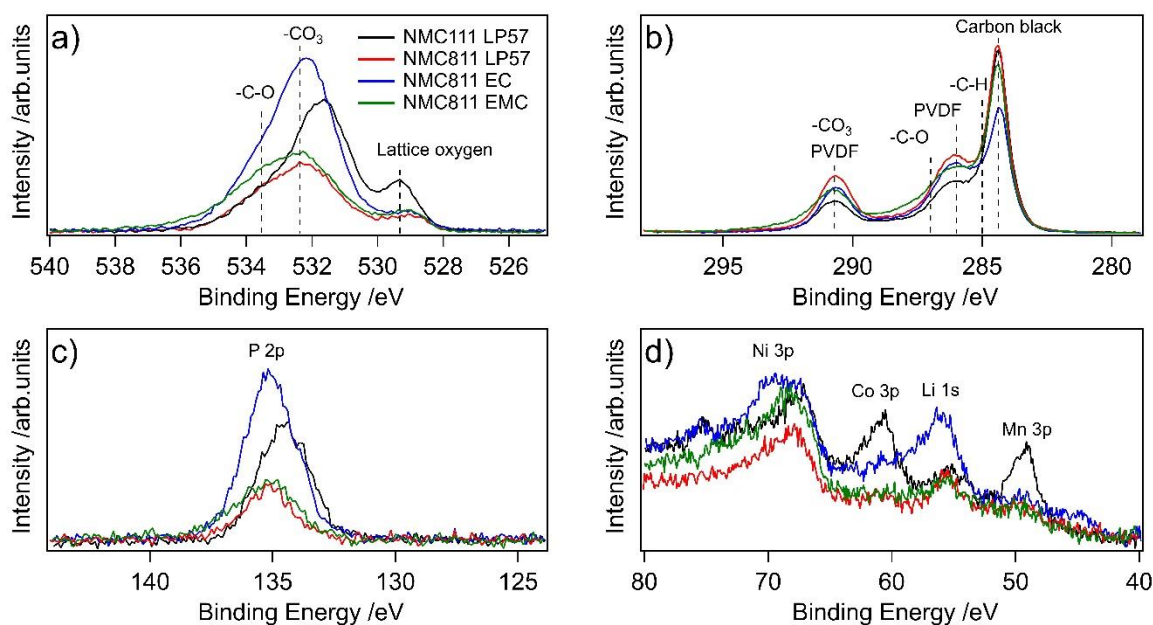
Figure 6. XPS spectra of NMC electrodes extracted from NMC/LTO cells after the first charge-discharge cycle between 1.45-3.05 V at C/20 with a 60 h potentiostatic hold at 3.05 V for NMC111 and 811 with electrolytes LP57, 1.5 M LiPF 6 in ethyl methyl carbonate (EMC),
