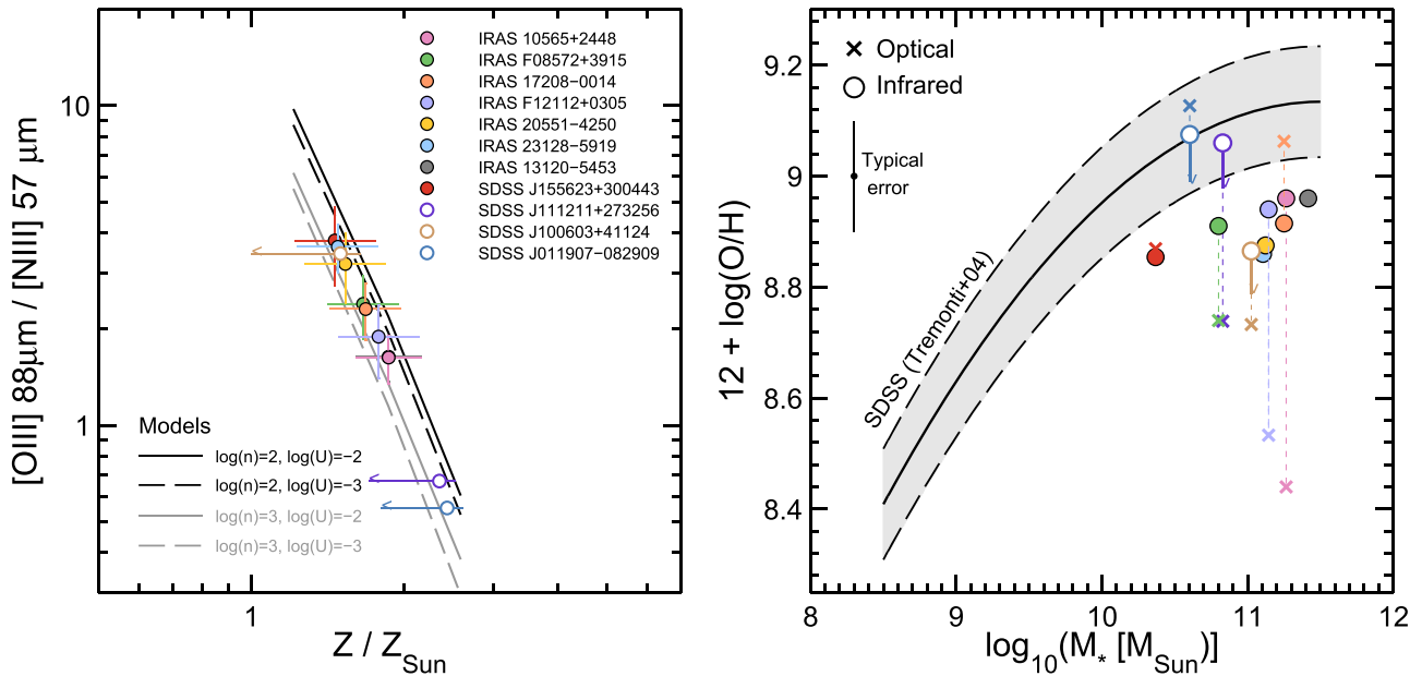
Figure 7. (Left) [O\text{ III}] 88\text{ }\mu\text{m}/[N\text{ III}] 57\text{ }\mu\text{m} emission line ratio as a function of metallicity based on the photoionization models reported in Pereira-Santaella et al. (2017; see also Nagao et al. 2011). The models (black and gray lines) assume ionized gas densities and ionization parameters in the 10^2\text{--}10^3\text{ cm}^{-3} and 10^{-3}\text{--}10^{-2} range, respectively. The observed [O\text{ III}] 88\text{ }\mu\text{m}/[N\text{ III}] 57\text{ }\mu\text{m} line ratio for 11 (U)LIRGs, and the corresponding abundance range expected from the model, are shown with filled circles when both lines are detected, and open circles when only the [O\text{ III}] 88\text{ }\mu\text{m} line is detected. (Right) Mass-metallicity relation observed in local galaxies (Tremonti et al. 2004) and (U)LIRGs whose metallicities are measured using optical-based (crosses; Tremonti et al. 2004; Rupke et al. 2008; Hou et al. 2009) and IR-based (circles; this work) methods. All metallicity measurements are shown in the Tremonti et al. (2004) scale. These results confirm that (U)LIRGs tend to have lower oxygen abundances compared to star-forming galaxies of the same stellar mass, but shows that this offset is smaller than previously thought from studies based on optical-based metallicities (e.g., Rupke et al. 2008).
