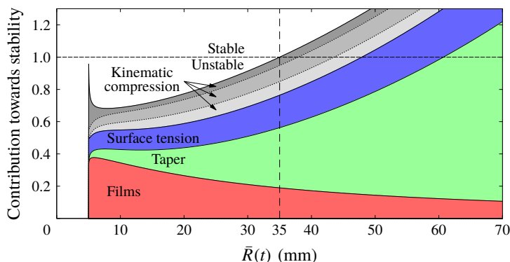
FIGURE 7. (Colour online) Evolution of the contribution towards stability of various physical mechanisms for n=13 (the last mode to decay) in the D56/H56 latex cell with Q=Q_{35} (see table 1), as a function of the average radius \bar{R} . The magnitude of each of the four terms in (3.18) is shown with a coloured band and their cumulative total indicates the contribution towards stability. Stability is achieved if the sum of these contributions is greater than or equal to 1. The kinematic-compression term is further subdivided according to the three terms in (3.19), again in order from bottom to top.
