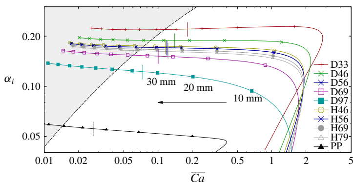
FIGURE 8. (Colour online) Numerically calculated evolution of the capillary number and taper angle (i.e. the slope of the sheet at the interface) for each cell in table 1 with Q=Q_{35} . The arrow indicates the direction of the evolution, and the symbols indicate when \bar{R}=10 mm, 20 mm, etc. The vertical bars show \bar{R}=35 mm where the system stabilizes according to the rigid-wedge model. The shaded region indicates where a rectilinear steady-peeling solution is stable (Peng & Lister 2018).
