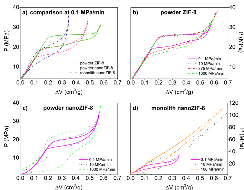
Figure 3. Room temperature PV-isotherms for the ZIF-8 + water system: (a) comparison between \text{powder}_{\text{ZIF-8}} , \text{powder}_{\text{nanoZIF-8}} , and \text{mono}_{\text{nanoZIF-8}} at 0.1 MPa/min compression rate; (b) \text{powder}_{\text{ZIF-8}} , (c) \text{powder}_{\text{nanoZIF-8}} , and (d) \text{mono}_{\text{nanoZIF-8}} at different compression rates.
