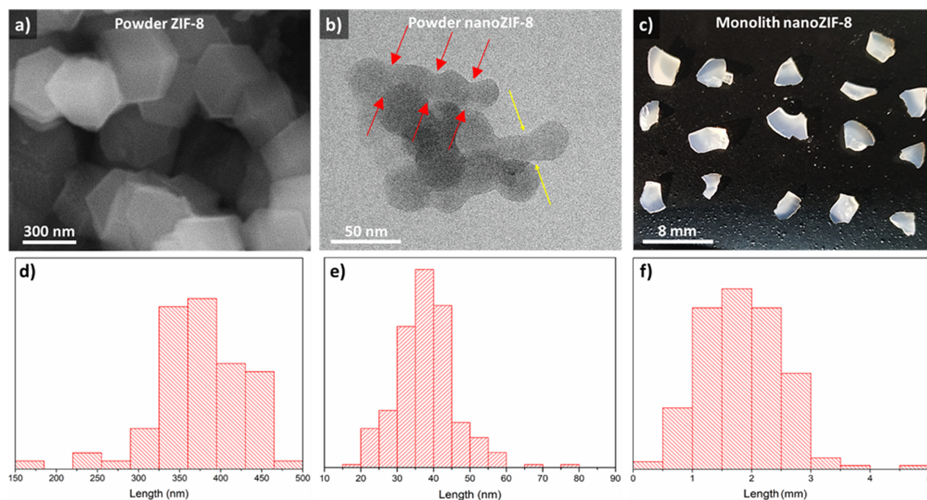
Figure 2. Representative images for different ZIF-8 samples: (a,d) SEM image and crystal size distribution for \text{powder\_ZIF-8} . (b,e) TEM image and crystal size distribution for \text{powder\_nano\_ZIF-8} ; here, the yellow arrows indicate GBs between crystals. The red arrows indicate GBs among a set of crystallites forming a \text{powder\_nano} grain; this case shows that for \text{powder\_nano} sample, crystallites are highly constrained from the formation of tight GBs. This is probably due to self-assembly of smaller crystallites preferentially exposing (110) surfaces, as discussed in ref 62. (c,f) Optical image and monolith size distribution for \text{mono\_nano\_ZIF-8} .
