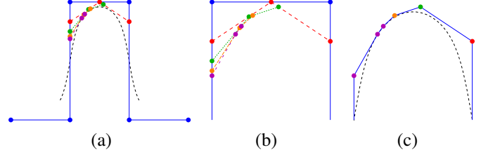
Figure 3: (a) A cubic B-spline curve (dashed black line), defined by the blue control polygon and knot vector [1, 2, 3, 4, 5, 6, 7, 8, 9, 10] . The curve is refined four times between the fifth and sixth knot value at 5\frac{1}{2} (red), 5\frac{1}{4} (green), 5\frac{1}{8} (orange), and 5\frac{1}{16} (purple). (b) A close-up view of the refinement steps. In each case a new control point is inserted and two existing points are moved. (c) One possible presentation of the user-interface, with the finest refinement presented to the user.
