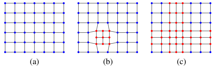
Figure 1: (a) A NURBS patch showing control points in a regular grid. (b) The desirable approach to local refinement, with new control points in a local area only. (c) Attempting to do this with NURBS introduces new control points across the mesh owing to the tensor product nature of NURBS patches.
