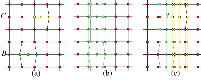
Figure A.10: (a) The user-interface presentation of a tensor-product NURBS patch (red) with two extra control points inserted, one on row B (green) and one on row C (yellow). In this cubic example, each newly-introduced point causes two other, existing, points to be replaced. Note: all figures in the Appendix show geometric space, not parameter space, with the red control points in a square grid before the insertions. (b) The layer corresponding to the point introduced on row B . Every row other than B requires three new points (shown in green) to be calculated from existing points. The replaced points are shown in grey. (c) The next layer down, corresponding to the point introduced on row C . There is a problem on row C .
