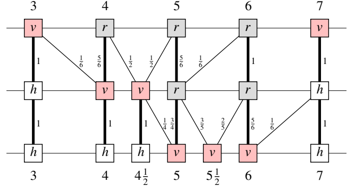
Figure 4: A one-dimensional example of the basic data structure. This example shows three layers of control points. The t value associated with each control point is shown at top and bottom of the diagram. The top row is the coarsest layer, defined by uniformly-spaced knot values; for example, the top-left point has a basis function defined by knots [1, 2, 3, 4, 5] . The central row shows the next layer, where the knot 4\frac{1}{2} has been inserted. The bottom row shows the third layer, where the knot 5\frac{1}{2} has been inserted. Each control point is marked as v ( visible ), r ( replaced ) or h ( hidden ). Thick connecting lines show parent-child relationships. Thin connecting lines show other relationships. Note that every point has a child (except in the lowest layer) but not every point has a parent. Weights on lines show how each hidden point is calculated from points in the layer above (and also how each of the other points was originally calculated from points in the layer above when the layer was created).
