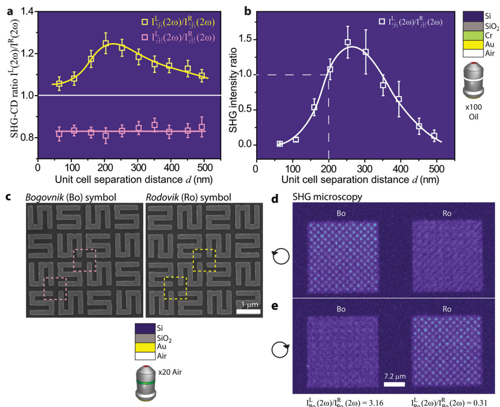
Figure 2. Optimizing the nonlinear chiroptical response of the meta-surface by gap size and design. (a), SHG-circular dichroism (SHG-CD) from the \mathbb{H} and \mathbb{R} chiral centers displayed as a function of the gap size d . (b), Ratio of SHG intensity I^L(2\omega)/I^R(2\omega) as a function of the gap size d . (c), SEM images of the Bogovnik (Bo) and Rodovik (Ro) traditional Slavic symbols. Contrary to the \mathbb{H}/\mathbb{R} geometry, the Bo/Ro geometry consists of identical (and not mirrored) interspaced unit cells. (d)-(e), SHG microscopy of the Bo and Ro sample arrays, upon illumination with left- and right-hand circularly polarized light, respectively.
