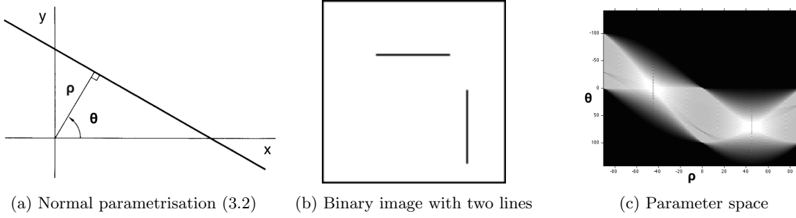
Figure 5: Normal form: image and parameter spaces.
