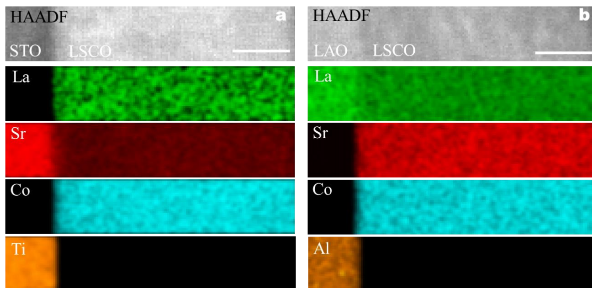
Supplementary Figure 1. HAADF images and corresponding EDX maps of the LSCO64 thin films deposited on (a) STO and (b) LAO substrates. The compositional maps demonstrate atomically sharp interfaces with the substrates in both cases. There are no any segregations of constitute elements.
