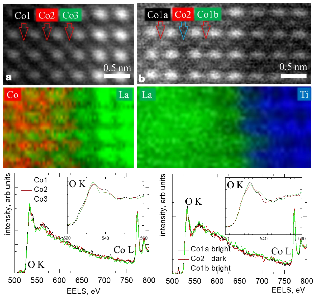
Supplementary Figure 2. HAADF images and corresponding EELS maps of the LSCO64 thin films deposited on (a) LAO and (b) STO substrates. At the bottom of the figure the EELS spectra for the selected Co atomic rows (shown on the top part of the figure) are shown.
