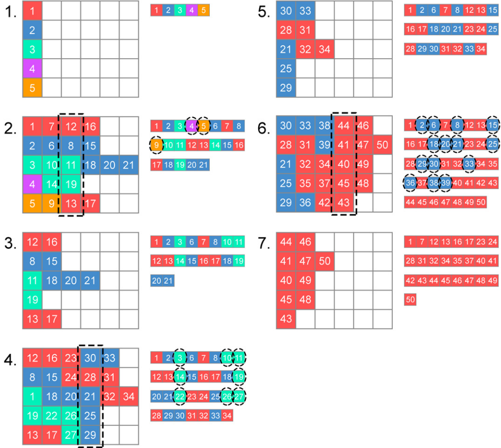
Figure 12. Sketch of the growth process for large corridors, with the spatial data structure carrying the pointers on the left and the data structure carrying the actual cell information on the right.
