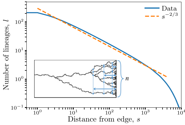
Figure 2. Number of surviving lineages in the genealogy of n individuals at the edge of the colony, traced backwards as a function of the distance s from the edge of the colony. Inset shows an example of a genealogy from an Eden model simulation. The shown plot was generated by averaging over the results of 120,000 simulation runs.
