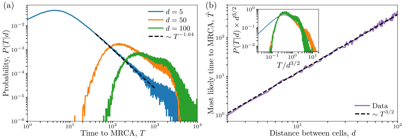
Figure 1. Left, probability distribution of time T to the most recent common ancestor for individuals sampled a distance d apart, for simulations in a linear corridor. Right, dependence of the most probable value \hat{T} of the distribution on the separation d . Inset shows the data on left, rescaled by the measured dependence of the peak of the distribution \hat{T} \sim d^{3/2} . The shown plots were each generated by averaging over the results of 600.000 simulation runs.
