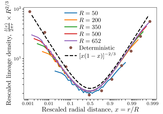
Figure 5. Lineage density as a function of distance from the colony center, rescaled by the final colony radius. The horizontal axis is a logit scale which reveals the power-law divergences in the lineage density as r/R \rightarrow 0 and r/R \rightarrow 1 . Solid lines are measured from Eden simulations at different final sizes R ; symbols are from the universal tree model with p = 4 ; dashed line is a phenomenological master curve (equation (11) with \epsilon = 1 ). The shown plots were each generated by averaging over the results of 48.000 simulation runs.
