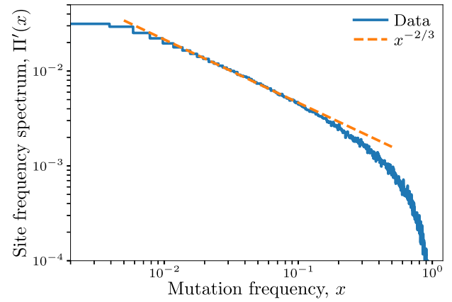
Figure 3. Site frequency spectrum, i.e. probability of a mutation attaining a frequency x , for individuals sampled from the edge of a population generated using Eden model simulations in a corridor geometry. The shown plot was generated by averaging over the results of 24,000 simulation runs.
