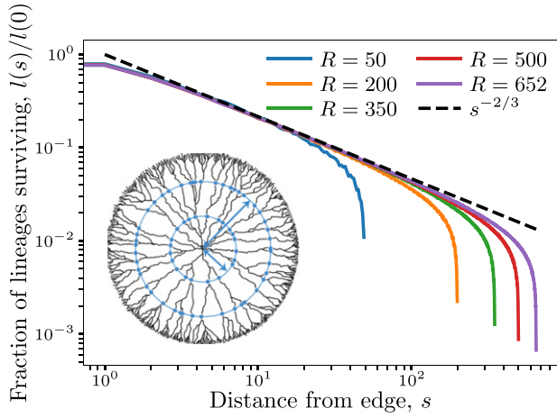
Figure 4. Fraction of lineages which survive when the genealogy of all individuals at the edge of the colony is traced inward, as a function of the distance s from the edge of the colony. Solid lines show data from radial Eden simulations grown to different final radii R . Dashed line shows expected decay based on lineage fluctuations in the KPZ class. Inset shows an example of a genealogy for a radial Eden simulation. The shown plots were each generated by averaging over the results of 48.000 simulation runs.
