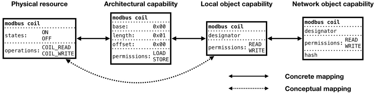
Figure 6.2: Relationship between a physical resource and its capabilities. Conceptually, the physical resource is represented by a single object capability; concretely, that object capability is constructed from one or more CHERI capabilities. The local and network object capabilities map in a 1:1 relationship.
