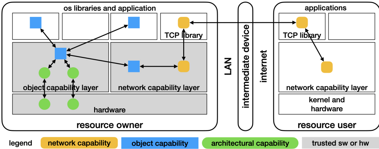
Figure 6.1: End-to-end design pattern for a distributed CPS capability system. This parallels the ‘automation cell’ architecture in Figure 5.1, where the resource owner is the PLC, the user is the workstation, the intermediate device is the modem or firewall, and each of these can issue commands to manipulate resources. In the capability architecture, only the shaded entities can create or modify capabilities to manipulate resources.
