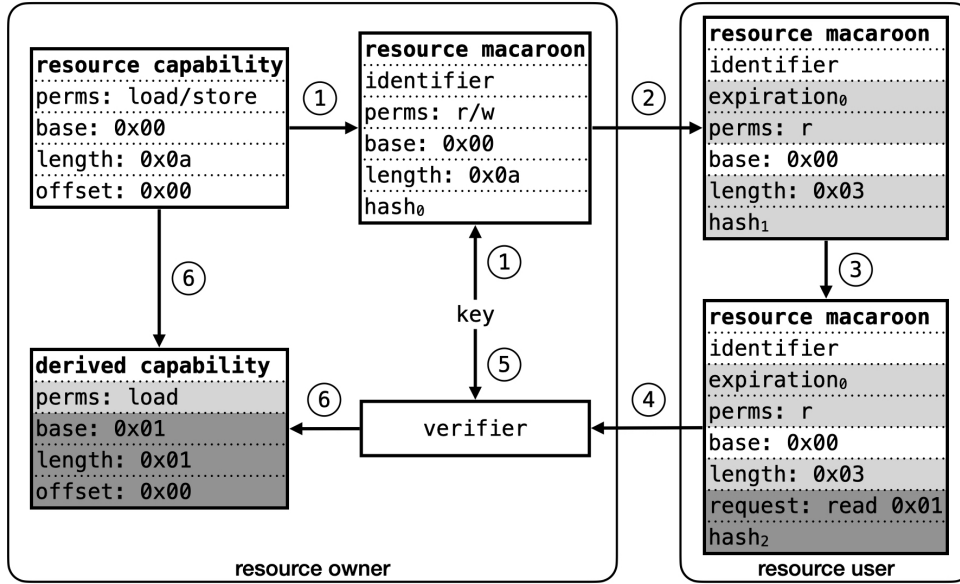
Figure 6.3: Composing distributed capabilities. The CHERI-based capability is mapped to a Macaroon-based capability (1). The Macaroon is provided to the resource user (2), who caveats the Macaroon with a request (3), and returns it to the owner (4). The owner verifies the Macaroon (5), derives an attenuated local capability (6), and invokes the resource using the derived capability.
