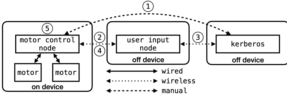
Figure 6.4: Architecture of the ROS case study. During provisioning, the motor control node shares a secret with Kerberos (1) to construct third-party Macaroons. At runtime, the motor control node generates and shares resource Macaroons (2). The user input node authenticates with Kerberos and receives a third-party Macaroon (3). The user input node caveats the resource Macaroon with the requested action, binds it to the third-party Macaroon, and returns both to the motor control node (4). Finally, the motor control node validates the Macaroons, derives a restricted CHERI capability, and executes the request (5).
