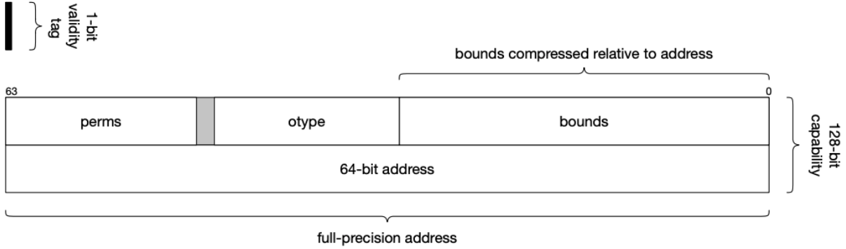
Figure 2.3: 128-bit CHERI capability with the memory address, bounds, metadata, and out-of-band validity bit for a 64-bit memory address [215]. Figure used with permission.
