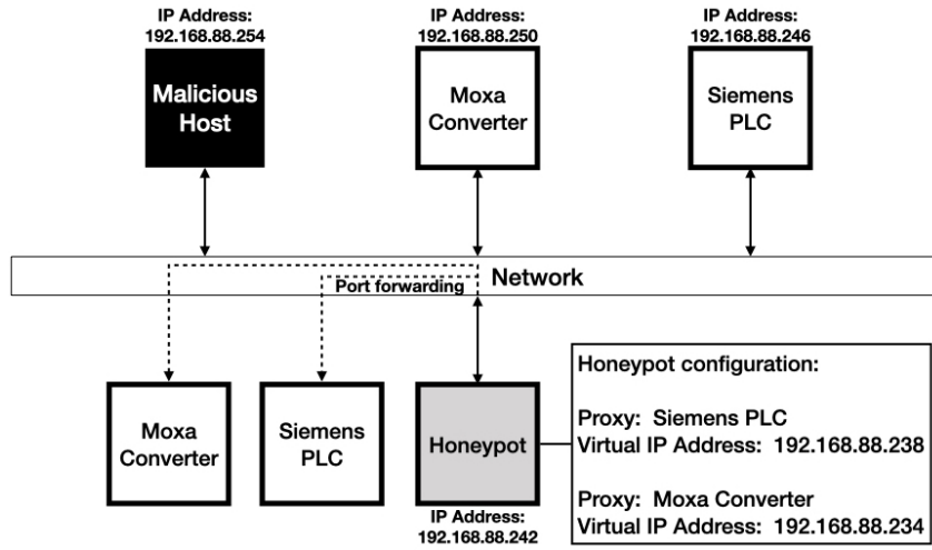
Figure 4.1: Sample deployment of a SecuriOT honeypot, showing the ability to emulate multiple virtual devices and act as a proxy for a custom device.
