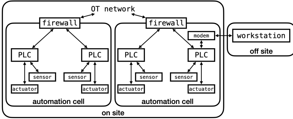
Figure 5.1: Example of an ICS ‘automation cell’ architecture [58].
