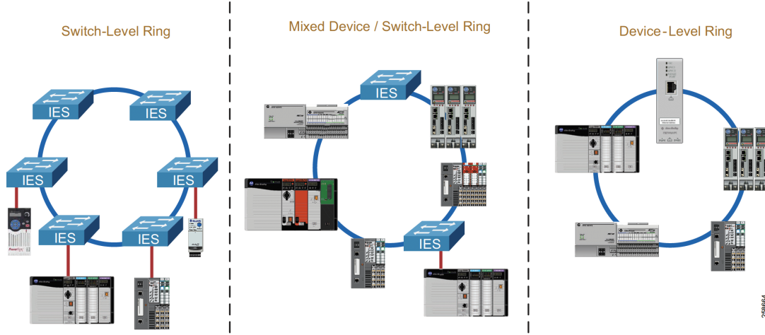
Figure 6.10: Rockwell Automation diagram showing multiple ring architectures [14].
