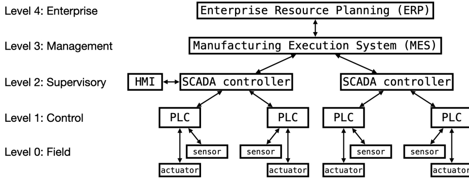
Figure 2.1: Simple example of a SCADA hierarchy.
