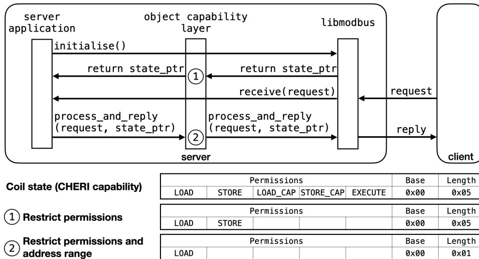
Figure 6.6: Example of the object capability layer minimising access to physical resources by limiting permissions and addresses accessible by libmodbus.
