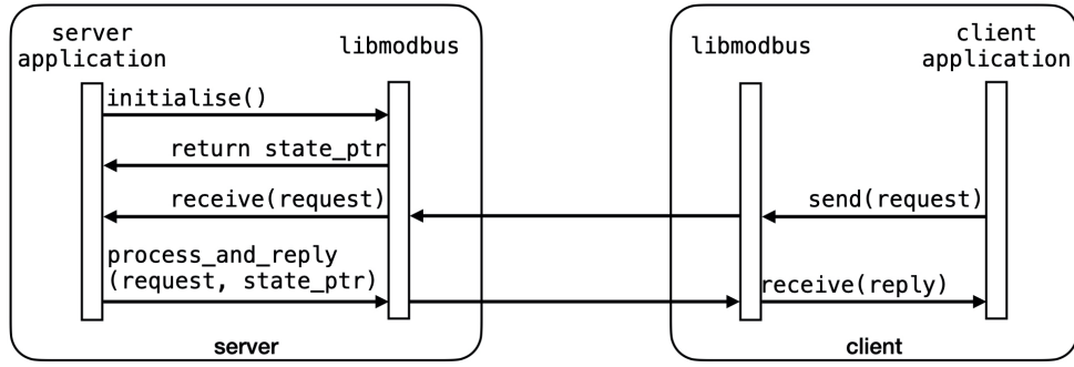
Figure 6.5: Example of initialisation and request/response interaction between applications and the libmodbus library.
