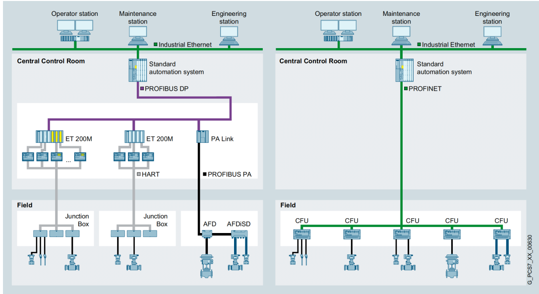
Figure 6.9: Siemens diagram comparing the multiple digital and analogue paths required by legacy field networks with CFU digitisation and consolidation [190].
