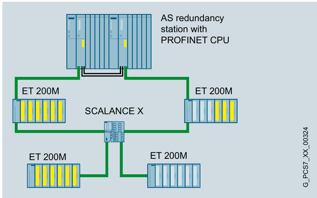
Figure 6.8: Siemens diagram showing redundant network transmission from redundant controllers [190].
