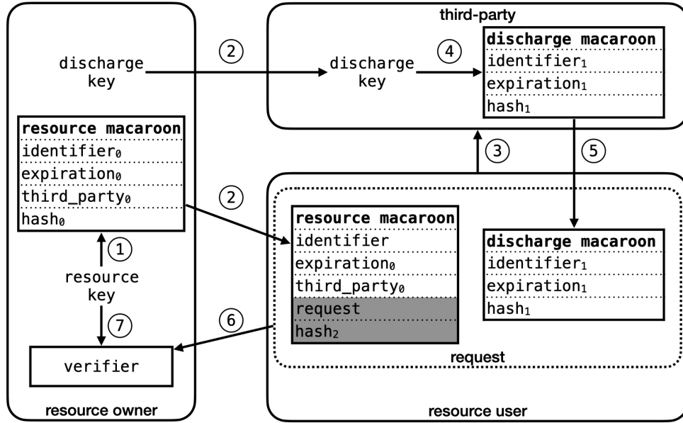
Figure 2.6: Example usage of a third-party Macaroon. The resource owner generates a resource key, used to create the initial resource Macaroon (1). The resource owner also creates a discharge key which is shared with the third party while the initial resource Macaroon is shared with the resource user (2). The resource user sends an authentication request to the third party (3). The third party uses the discharge key to generate a discharge Macaroon (4) and provides the discharge Macaroon to the resource user (5). The resource user applies the request as a caveat to the resource Macaroon and returns both Macaroons to the resource owner (6). The resource owner recursively verifies the resource and discharge Macaroons (7).
