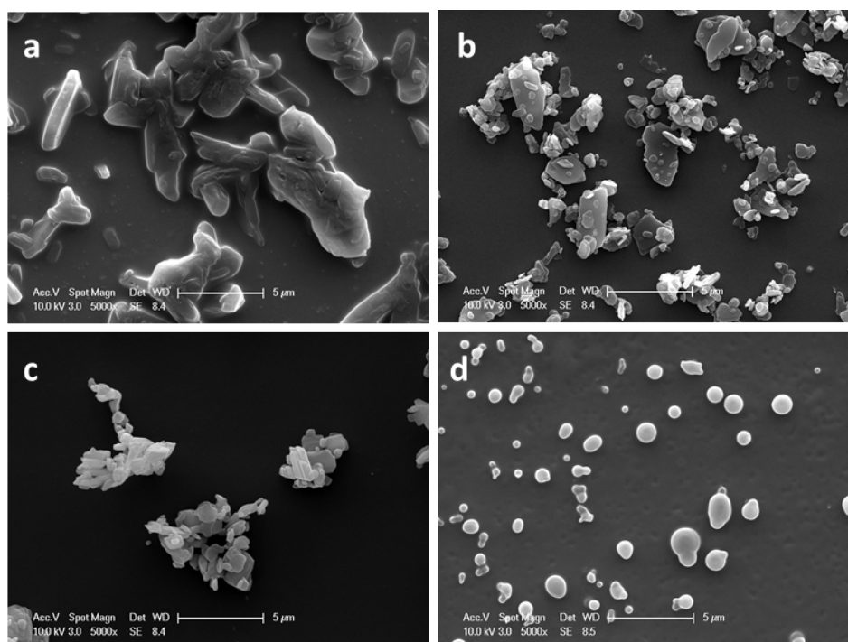
Figure 6 SEM images of: (a) salbutamol sulphate, (b) salmeterol xinafoate, (c) fluticasone propionate & (d) ciclesonide
