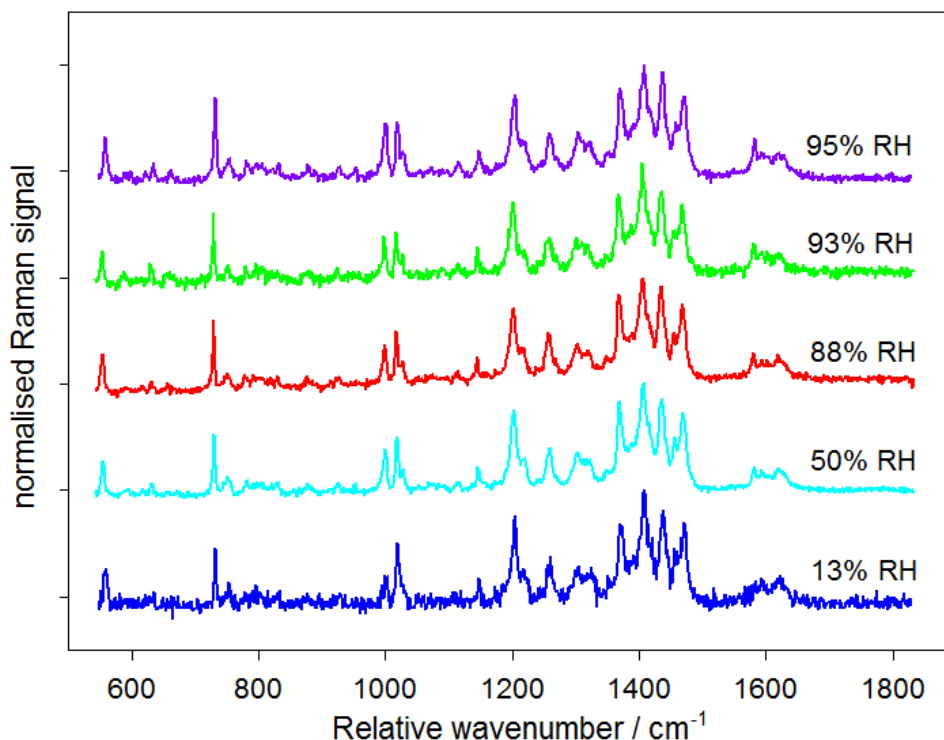
Figure 7 Raman spectra of salmeterol xinafoate at a range of RH values
