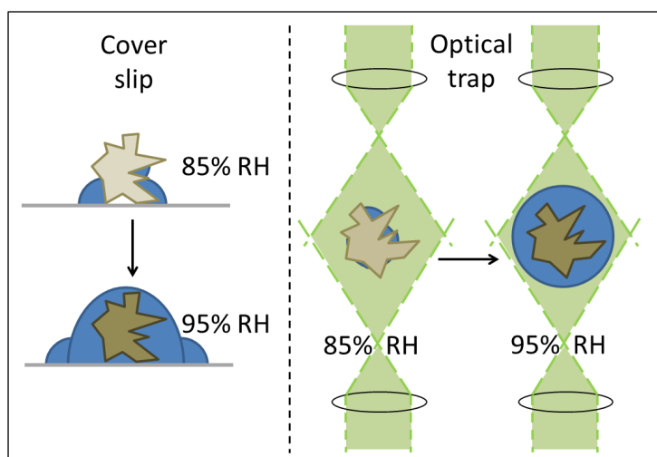
Figure 1. An illustration of the influence of coverslips on the formation of water layers on hygroscopic particles
