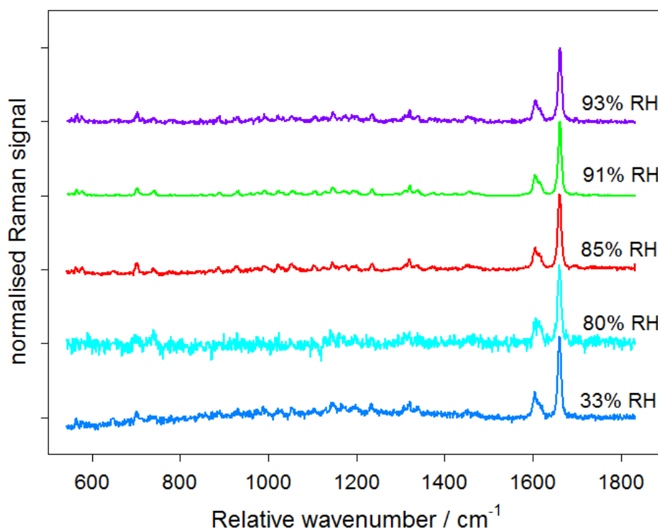
Figure 8 Raman spectra of fluticasone propionate at a range of RH values
