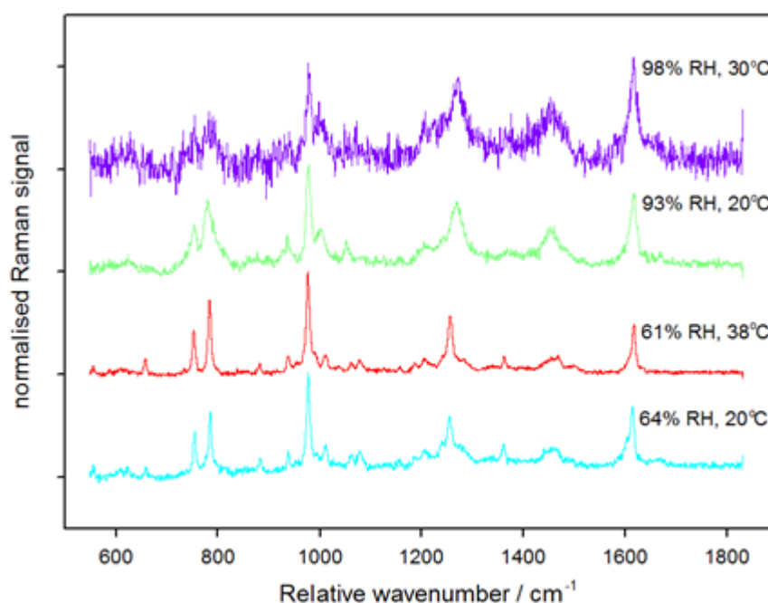
Figure 5 Raman spectra of optically trapped salbutamol sulfate particles at a range of RH and temperatures
