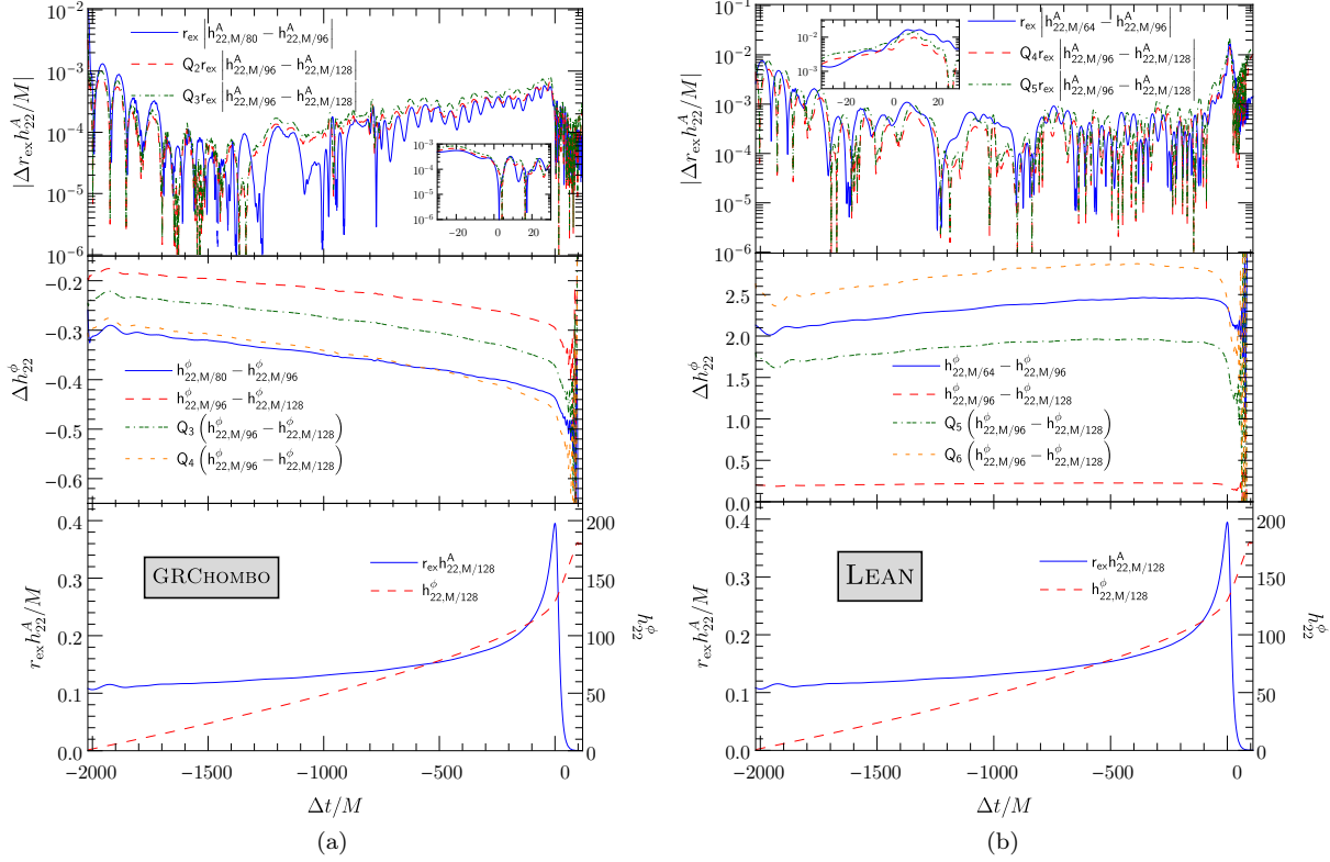
Figure 3. Convergence of the quadrupole mode of the strain h_{22} = -h_{22}^+ + ih_{22}^\times calculated from the values of \Psi_4 extracted for configuration q1-d12 at r_{\text{ex}} = 120 M for both GRCHOMBO with finest grid resolutions \Delta x_{\text{imax}} = M/80, M/96 and M/128 (a) and LEAN with finest grid resolutions \Delta x_{\text{imax}} = M/64, M/96 and M/128 (b). Top panels: Convergence of the amplitude h_{22}^A = |h_{22}| . The difference between the higher resolution results is rescaled according to fourth and fifth order convergence for LEAN and according to second and third-order convergence for GRCHOMBO. In each case, the inset shows an interval around the peak amplitude. Middle panels: Convergence of the phase h_{22}^\phi = \text{Arg}(h_{22}) . The difference between the higher resolution results is rescaled according to fifth and sixth order convergence for LEAN and third and fourth order convergence for GRCHOMBO. Bottom panels: For reference we plot the amplitude h_{22}^A and the phase h_{22}^\phi of the highest resolution waveform on the same time axis. For the two lower resolution waveforms from each code, we have time-shifted each of them in order to maximize the overlap (cf. (65)) with the highest resolution waveform. \Delta t = 0 corresponds to the maximum in h_{22}^A for the highest resolution waveform.
