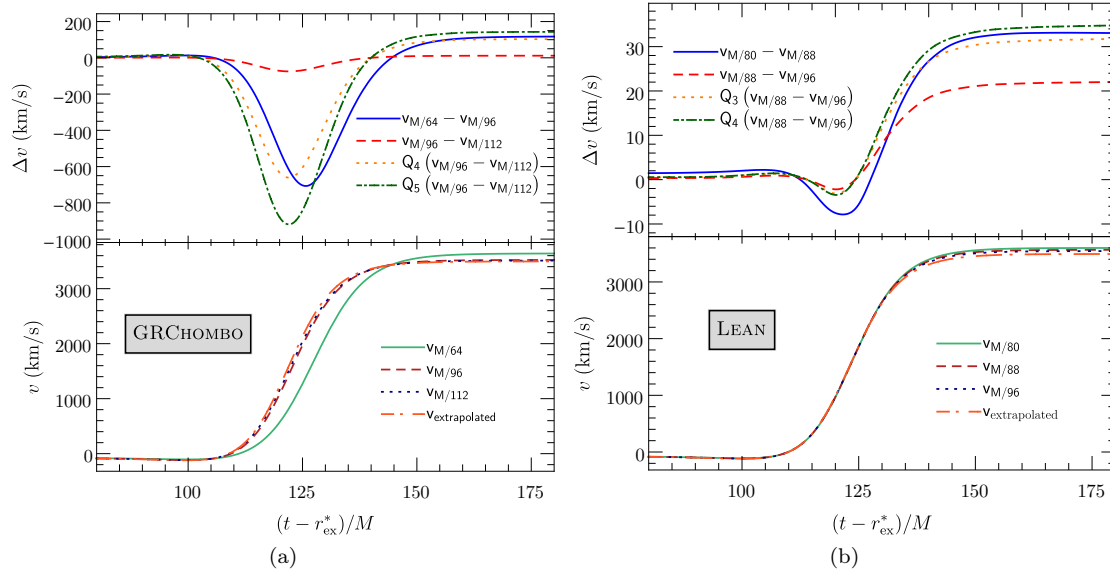
Figure 6. Convergence plots for the accumulated linear momentum radiated from configuration q1-s09 for GRCHOMBO with finest grid resolutions \Delta x_{l_{\max}} = M/64 , M/96 and M/112 (a) and for LEAN with finest grid resolutions \Delta x_{l_{\max}} = M/80 , M/88 and M/96 (b). This is shown in the form of the BH recoil velocity in the bottom panels. For both codes, the radiated linear momentum is calculated from the extracted \Psi_4 values at r_{\text{ex}} = 90M , and the extrapolated curve corresponds to a Richardson extrapolation assuming fourth order convergence. In the top panels, we show the difference between the results from different resolutions with rescalings according to third and fourth order convergence for LEAN and according to fourth and fifth order convergence for GRCHOMBO.
