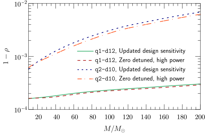
Figure 5. The discrepancy 1 - \rho between the (\ell, m) = (2, 2) mode of the gravitational wave signal from the q1-d12 (10 orbits, non-spinning, equal mass) and q2-d10 (6 orbits, non-spinning, 2 : 1 mass ratio) BH binary configurations simulated with LEAN and GRCHOMBO . For q1-d12 , we use the simulation with resolution \Delta x_{l_{\max}} = M/128 for both codes and for q2-d10 , we use the simulation with resolution \Delta x_{l_{\max}} = M/96 for both codes. For each configuration, we show the difference computed with the updated Advanced LIGO sensitivity design curve ( aLIGODesign.txt in [129]) and the zero detuned, high power noise curve from the Advanced LIGO anticipated sensitivity curves ( ZERO_DET_high_P.txt in [130]).
