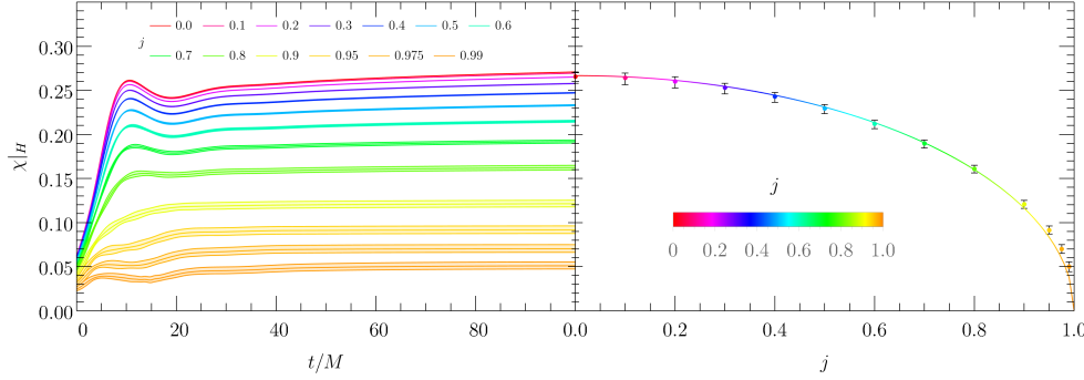
Figure C1. Plots illustrating the dependence of the value of the conformal factor \chi on the apparent horizon surface H in the moving puncture gauge (28), (30)-(31) for different values of the dimensionless spin j . For all plots, we use the quasi-isotropic Kerr initial data described in section 2.1.2 and the default values of the gauge parameters (29) with M\eta = 1 . Although we would expect the plots to vary for different gauge parameters (in particular, as \eta is varied), these plots provide a rough rule-of-thumb. The left panel shows the mean value of \chi as a function of time with the error bands around each curve corresponding to the maximum and minimum on H . The right panel shows the mean value of \chi over the interval t/M \in [40, 100] for each j with the error bars corresponding to the minimum and maximum values of \chi over the same interval. Furthermore, we show a fit of the mean value of \chi against j which takes the form \langle \chi \rangle_H \simeq 0.2666\sqrt{1-j^2} .
