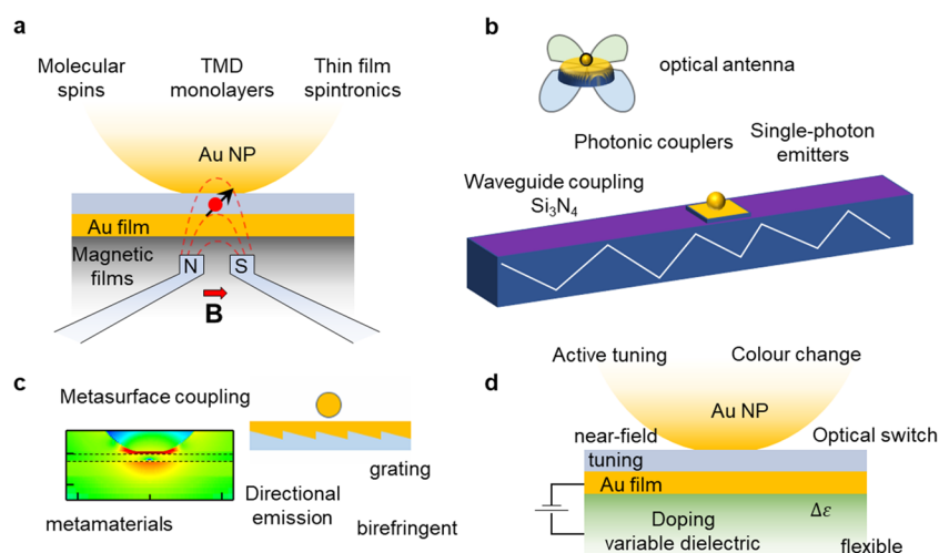
Figure 5. Utilization of NPoF geometry. (a) Coupling of magnetic and plasmonic spin systems. (b) Waveguide integration of NPoFs for single emitters, SERS sensing, and quantum information. (c) Photonic modification of thin metal surface allows coupling of a metasurface to a nanocavity. (d) Doping of underlying dielectric medium changes the MIMI modes and tunes the color as MIMI mixing occurs for d \approx 10 nm gaps.
