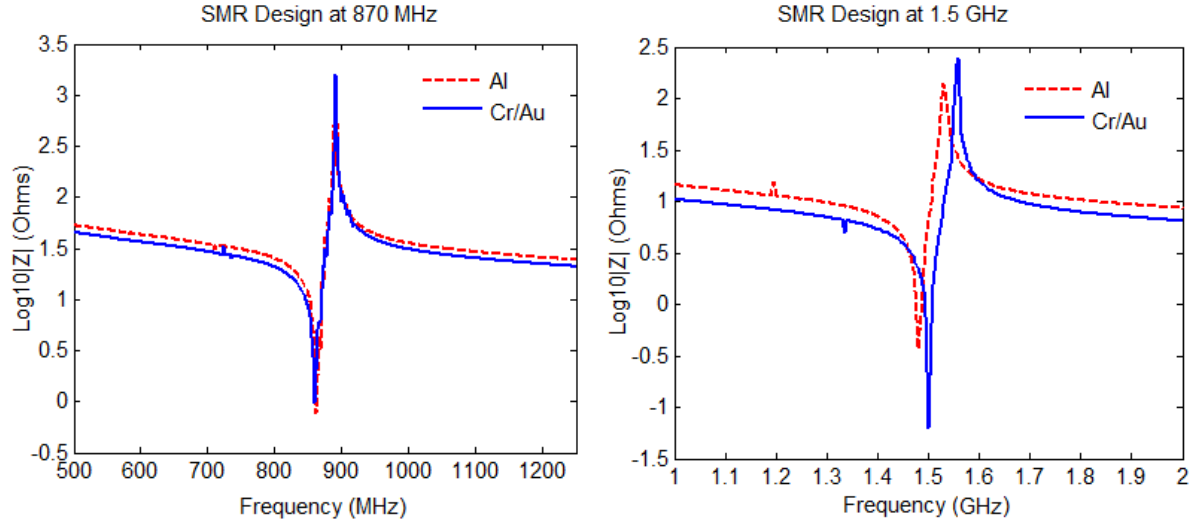
Figure 4. Frequency response of the designed SMRs modelled using a 2D finite element model.
