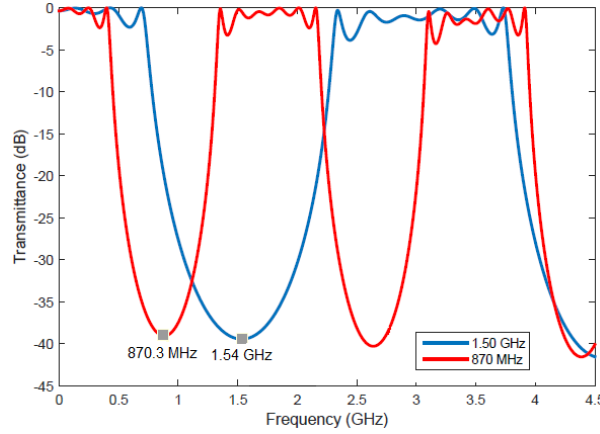
Figure 3. Simulated transmittance of the reflector stack consisting on 3 pairs of Mo/SiO 2 layers based on the Mason model.
