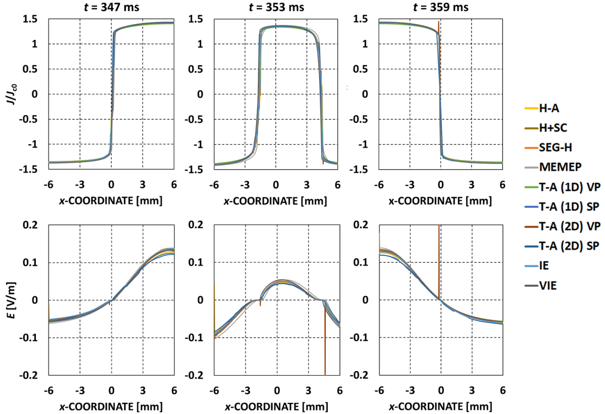
Figure 5. Distributions within the wire for: current density normalised to J_{c0} , J/J_{c0} , and electric field, E . The calculated distributions are shown for three key PM positions: (1) as the magnet approaches the centre of the wire from the right-hand side ( t = 347 ms in the 2nd cycle); (2) when the magnet is aligned with the centre of the wire ( t = 353 ms); and (3) as the magnet moves away from the wire on its left-hand side ( t = 359 ms). The dynamics of the current flowing within the wire and the related local electric fields ultimately give rise to the voltage waveforms shown in Figure 3
