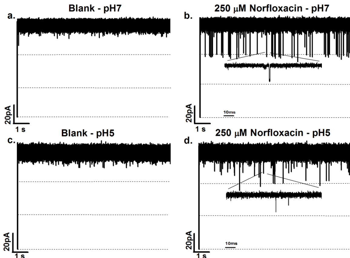
Figure 2. Ionic current traces of a single trimeric OmpF porin: (a) in the absence of antibiotics at pH 7, (b) with 250 \mu M norfloxacin cis side at pH 7, (c) in the absence of antibiotics at pH 5 and (d) with 250 \mu M norfloxacin cis side at pH 5. Electrolyte conditions: 1 M KCl, 5 mM acetate (pH 5) or 5 mM \text{PO}_4 (pH 7). The applied voltage was -25 mV. The dotted lines specify the ionic current levels through single monomers of the OmpF trimer. The addition of norfloxacin at pH 7 (b) leads to well resolved blockages of the ionic current through a monomer, whereas at pH 5 (d) the antibiotic molecules lead to flickering in the ionic current through a monomer – full blockages are not always observed. This is due to the low residence time of the antibiotic in the channel at pH 5, as discussed in the text.
