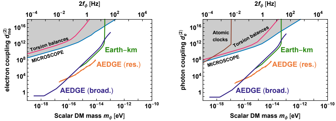
Figure 2. The sensitivities of AEDGE in broadband (purple lines) and resonant mode (orange lines) to quadratic scalar DM interactions with electrons (left) and photons (right), compared to those of a km-scale terrestrial experiment (green lines). The grey regions show parameter spaces that have been excluded by the MICROSCOPE experiment (blue lines) [20, 21], searches for violations of the equivalence principle with torsion balances (red lines) [22, 23], or by atomic clocks (brown lines) [24, 25].
