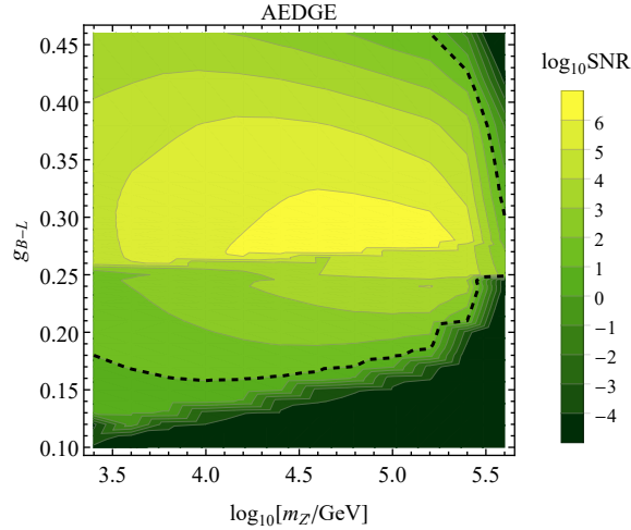
Figure 7. Signal-to-noise ratio (SNR) achievable with AEDGE in the parameter plane of the classically scale-invariant extension of the SM with a massive Z' boson. The dashed line is the \text{SNR} = 10 contour.
