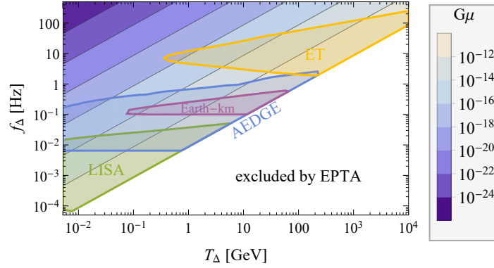
Figure 9. Frequency f_\Delta at which features in the cosmic string GW spectrum appear corresponding to events in the early universe occurring at the indicated temperature T_\Delta . The shading contours indicate G\mu values of the cosmic string network, and the reach of different experiments are indicated by the coloured regions.
