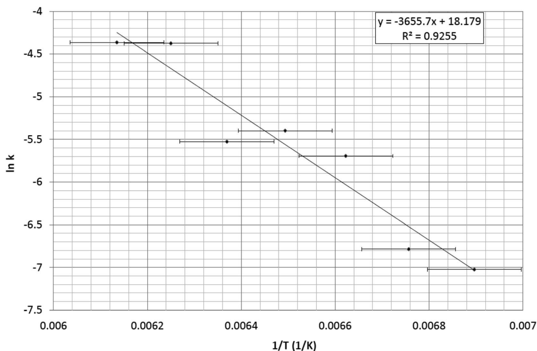
Fig. 4 Arrhenius plot of 1/T versus \ln k whose gradient ( E_a/R ) yields an activation energy, E_a = 30(1) \text{kJ mol}^{-1} .
